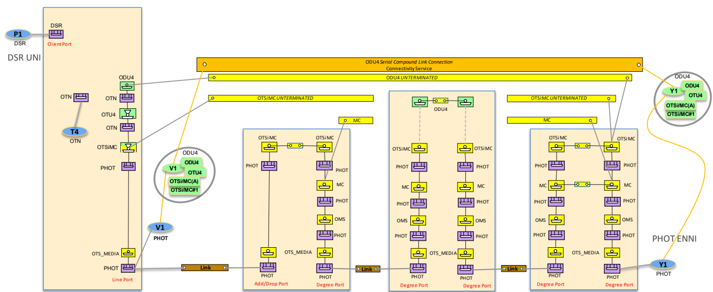
Figure 6-58 ODU Asymmetric scenario without ODU CS in the OLS subnetwork
