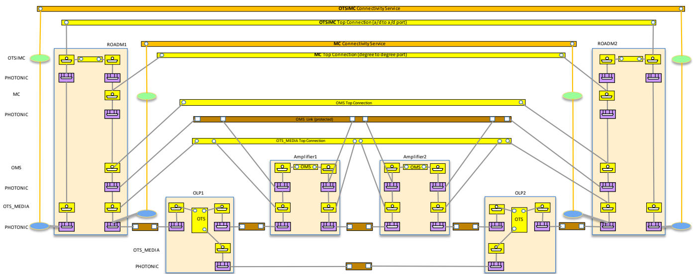
Figure 6-89 UC-5a OLP protection TAPI representation 2, with two amplifiers in Route 1
