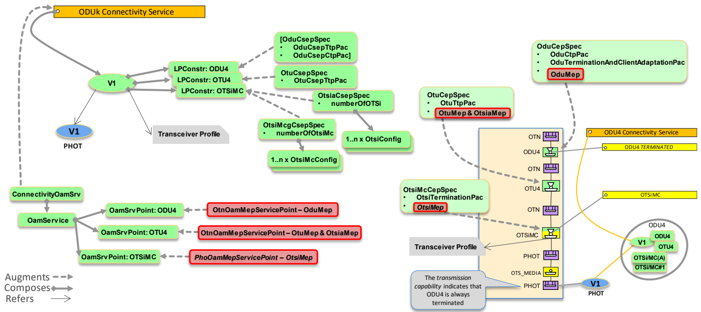
Figure 6-39 ODUk Trail Connectivity Service
