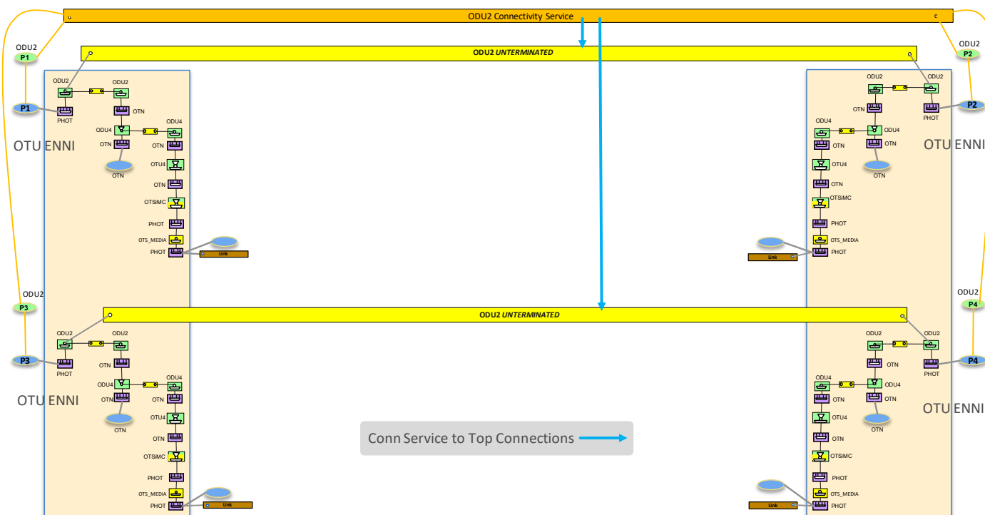
Figure 5-20 - Unterminated ODUk Service - Relationships between CSs and Top Connections
