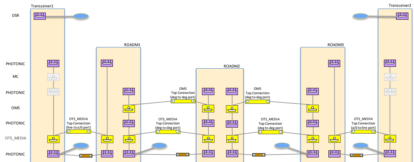
Figure 5-42 illustrates a possible layering for an integrated management scenario at time zero, with the (MC) SIPs at ROADM1 and ROADM3 degree ports.
