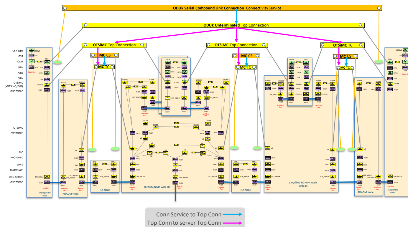
Figure 5-19 - 3R - Relationships between Connectivity Services and Top Connections
