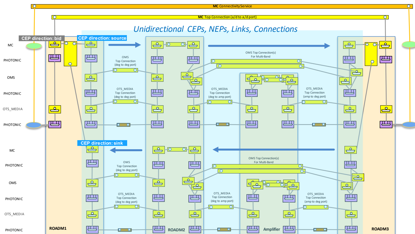
Figure 6-69 Mixed Scenario - UNI bidirectional and OMS unidirectional.
