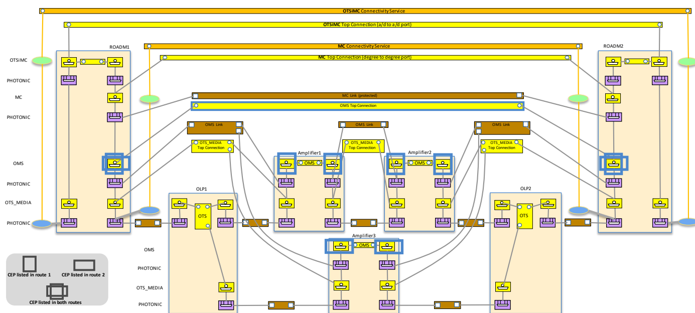
Figure 6-94 UC-5a OLP protection TAPI representation 3, OMS routes
