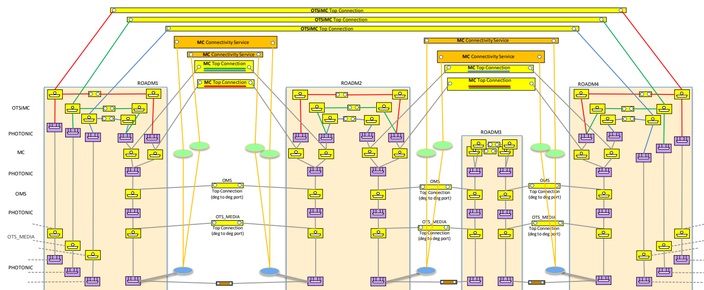
Figure 5-49 Scenario 2 : Integrated Management, sequence of MC top-connections
