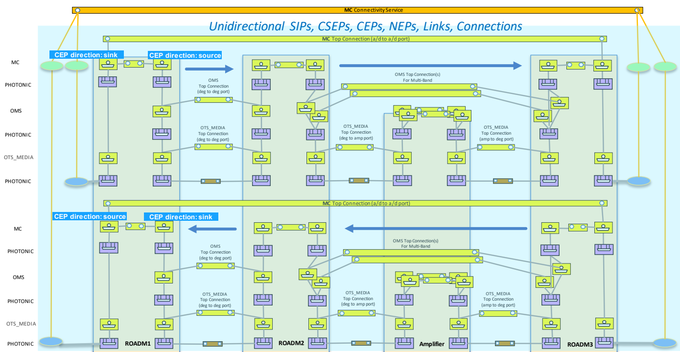
Figure 6-70 Full Unidirectional - UNI and OMS unidirectional scenario.
