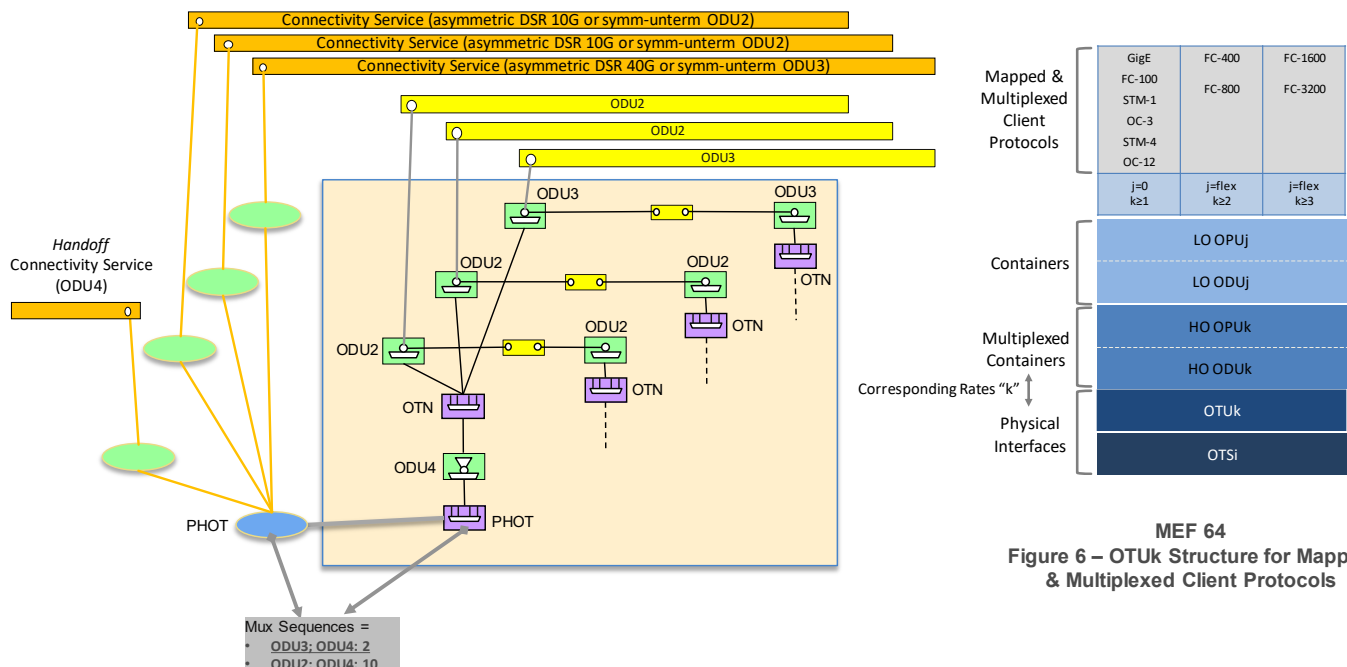
Figure 5-64 OTN ENNI, mapped &amp; multiplexed client protocols
