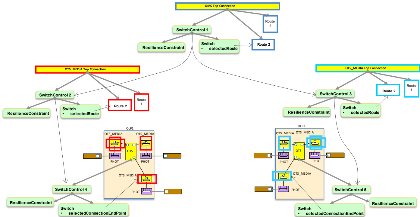
Figure 6-98 UC-5a OLP protection, state details
