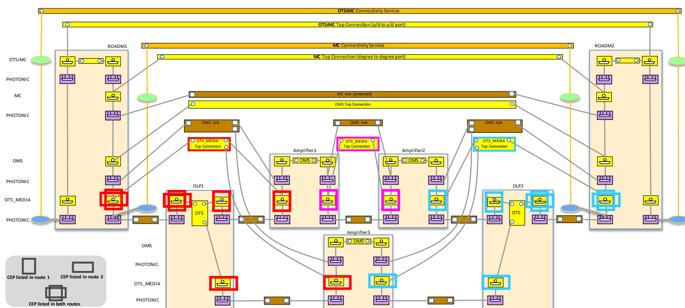
Figure 6-93 UC-5a OLP protection TAPI representation 3, OTS_MEDIA routes
