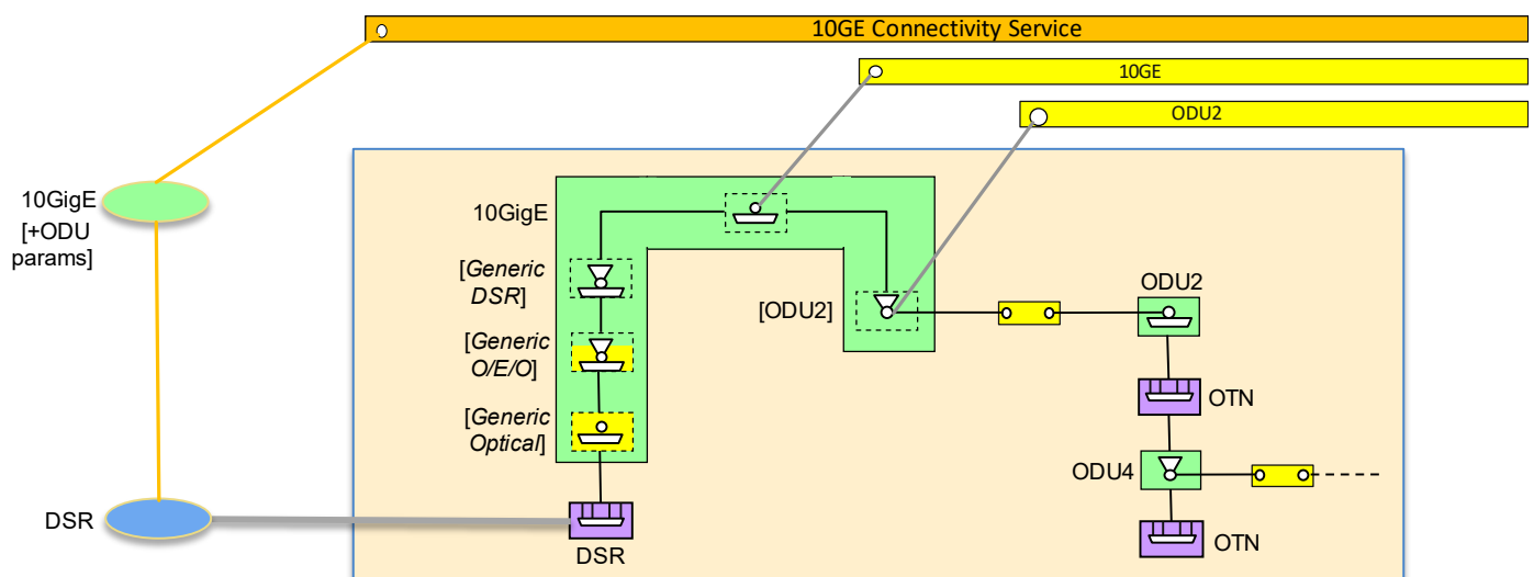
Figure 5-56 Option: Simplified DSR UNI with additional embedded functions
