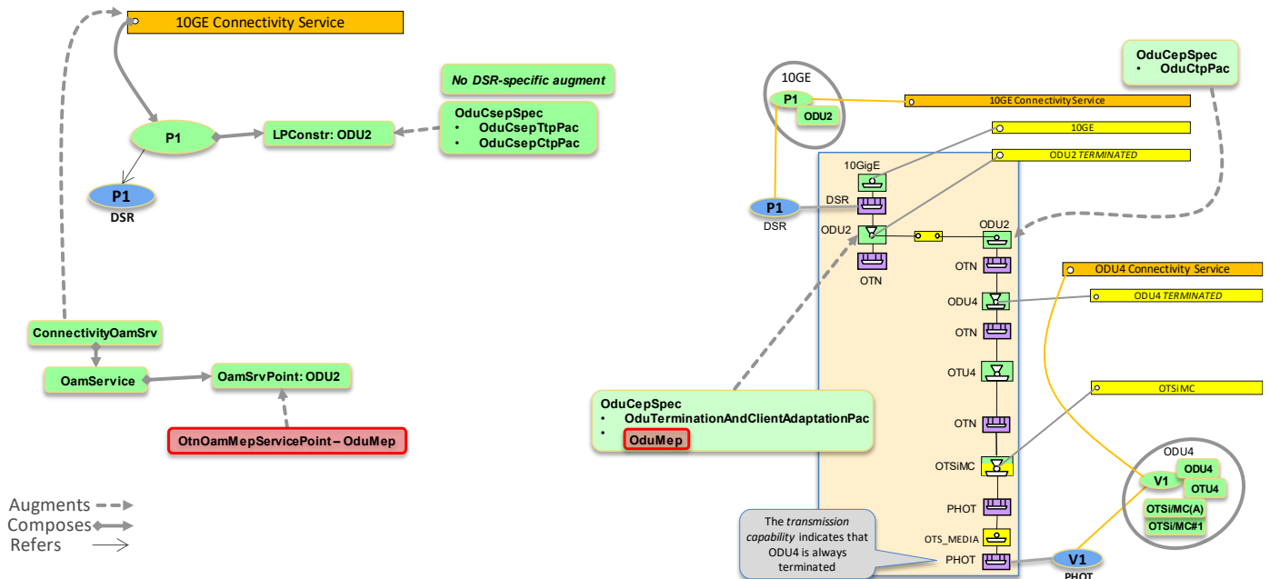
Figure 6-40 DSR/ODUj CS on ODUk CS
