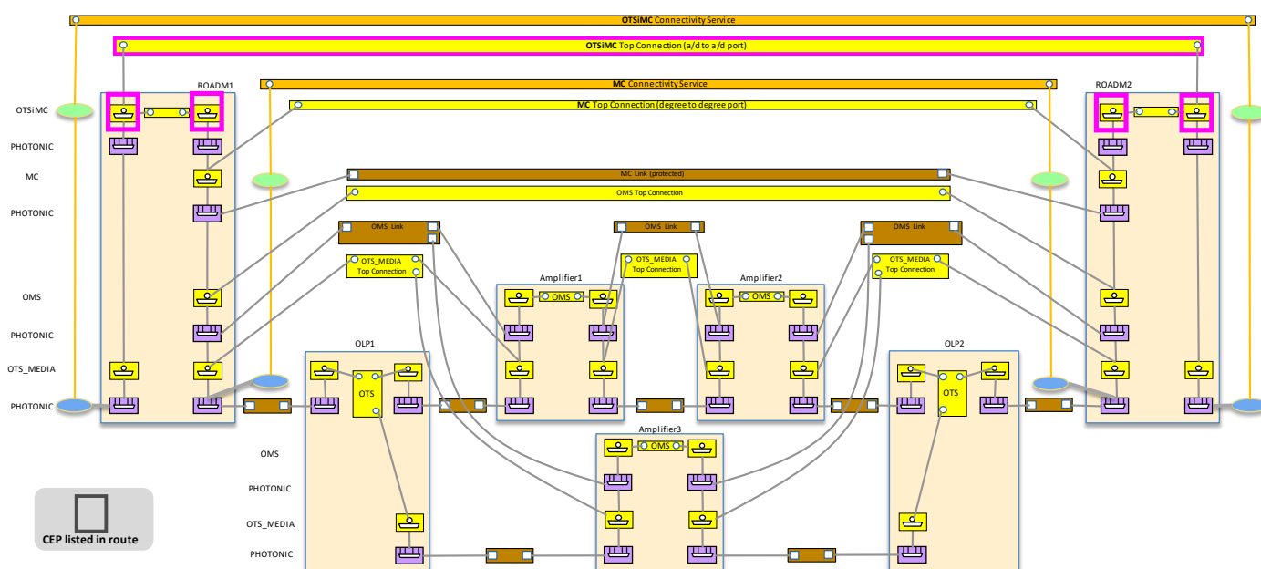
Figure 6-95 UC-5a OLP protection TAPI representation 3, OTSiMC route
