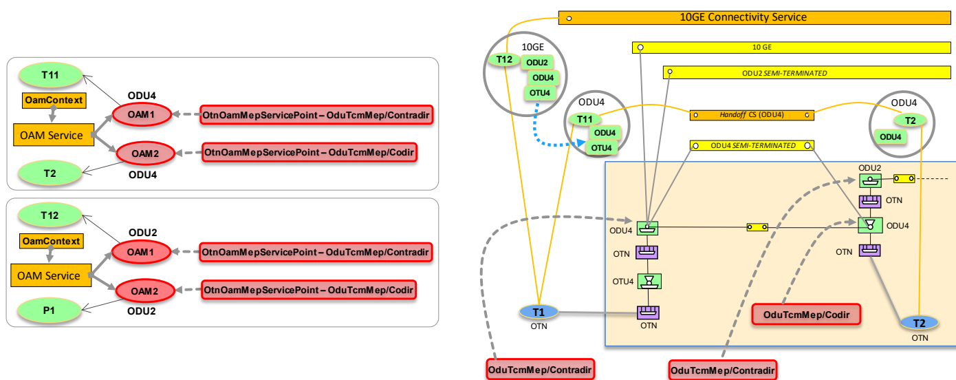
Figure 6-28 Asymmetric scenario 2: DSR/ODUj CS (OTN ENNI) - Auto creation of ODUk Handoff CS – Part 1
