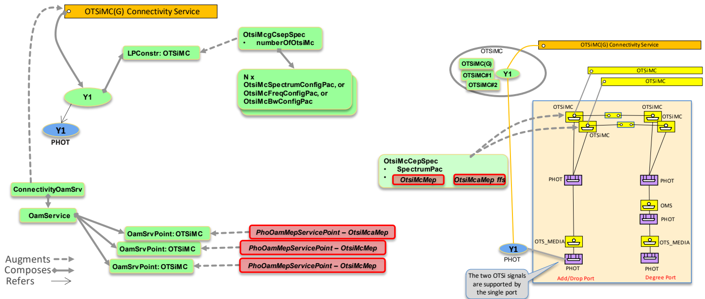
Figure 6-54 OTSiMC Connectivity Service without MC Layer
