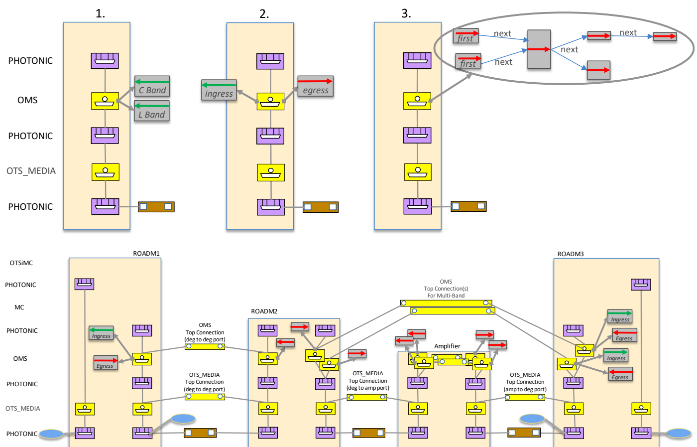
Figure 6-60 OMS CEPs and Amplification Functions
