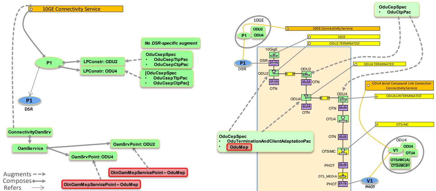
Figure 6-10 DSR/ODUj CS on ODUk SCLC CS, ODUk Terminated Connection automatically created or reused
