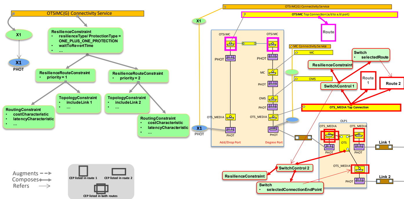
Figure 6-97 UC-5a OLP protection, provisioning and state details
