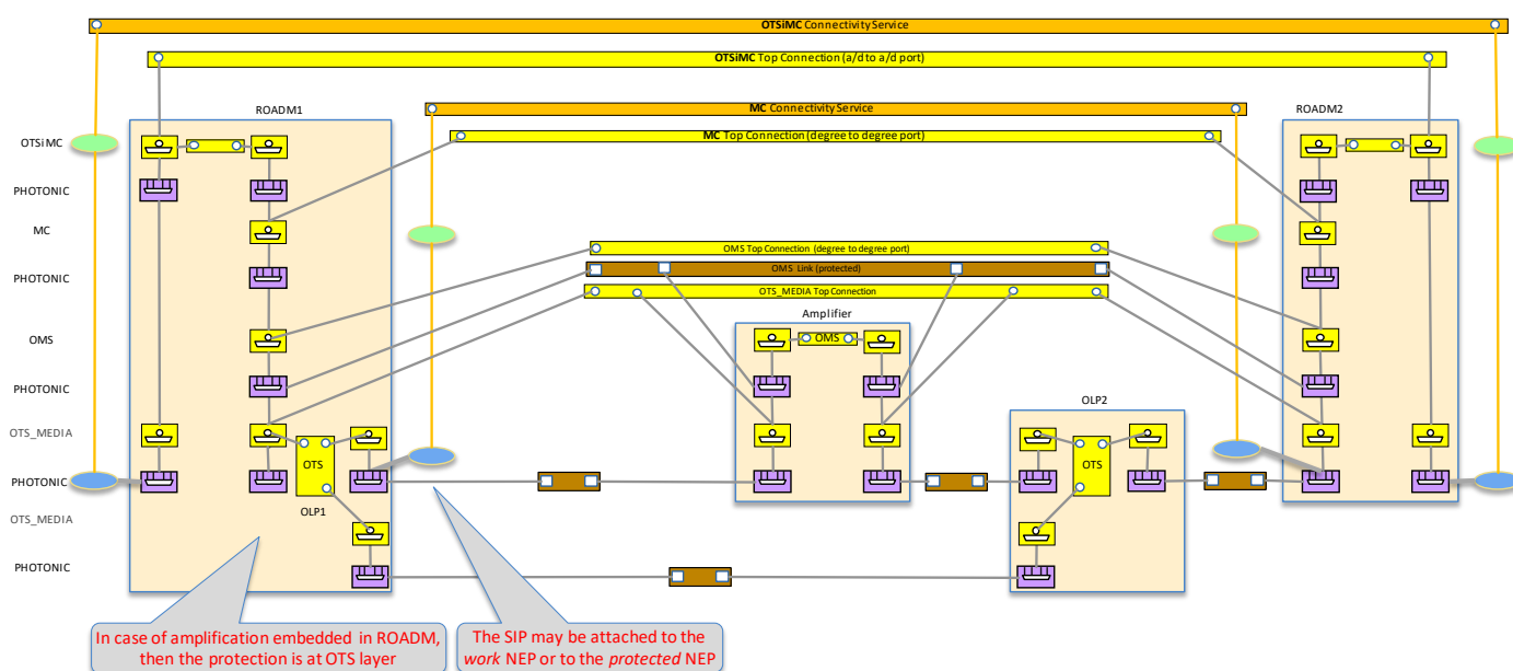
Figure 6-96 UC-5a OLP protection TAPI representation 4, with OLP function embedded in ROADM1
